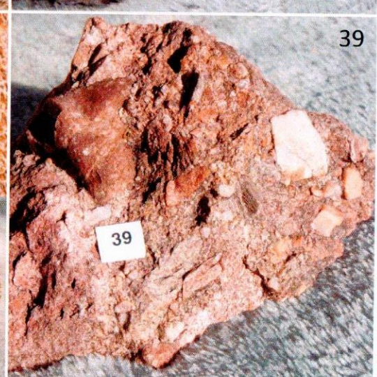
19 limestone 39 conglomerate
