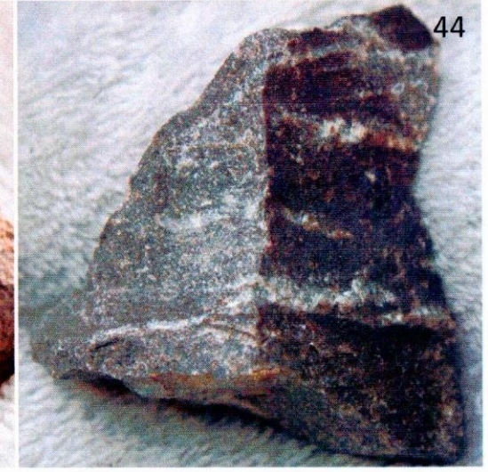
27 schist 44 quartzite
