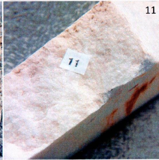
17 slate 11 marble
